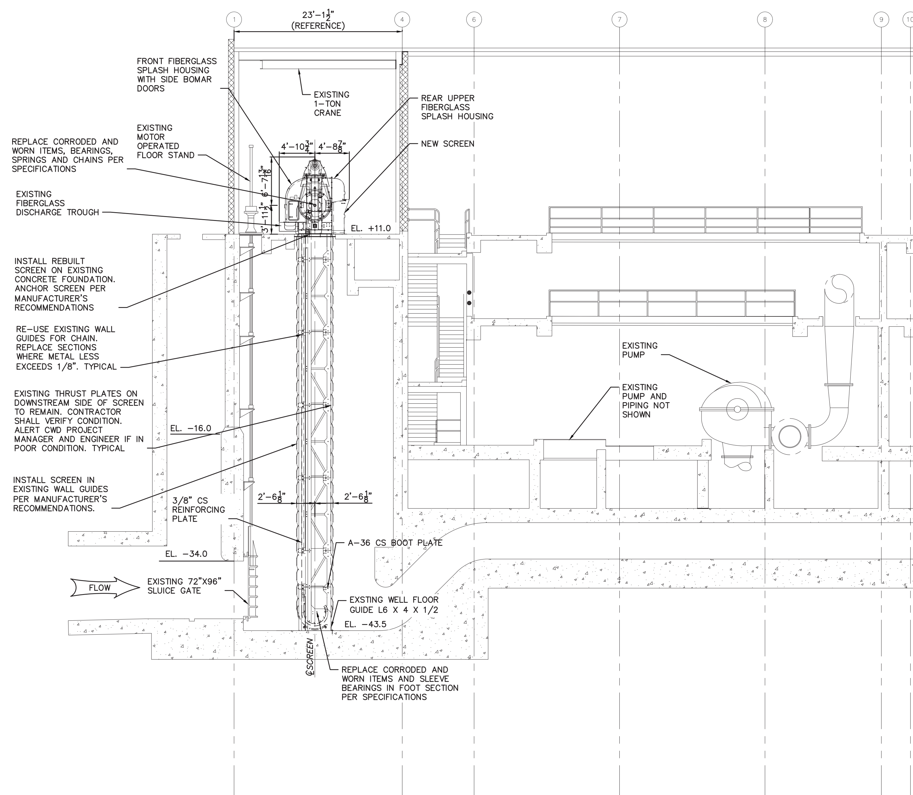
A M-4 SCREEN INTAKE SECTION VIEW SCALE: 1/8"=1'-0"
